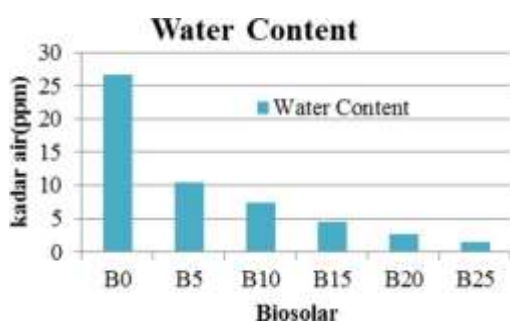
Gambar 4. Pengaruh Biosolar Terhadap Kadar Air (Water Content)
